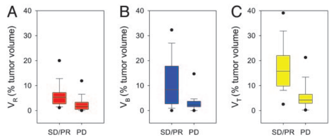
Fig. 3. Box plots summarizing fDM tumor volumes as a percentage of total tumor volume for each patient group, PD ( n = 15 ) and SD/PR ( n = 14 ). (A) The volumes (percentage of total) within the tumors that experienced significantly increased diffusion values ( V_R ). (B) The results for the tumor volumes that had a significant decrease in diffusion values ( V_B ). (C) The total volume of tumors that had any significant change in ADC ( V_T , where V_T = V_R + V_B ). Values depicted are the median for each group with the upper and lower limits of the box representing the 75th and 25th percentile, respectively. The error bars represent the 95th and the 5th percentiles. The dots are the limits (maximum and minimum) of the data range. P values (Student's t test, unpaired, two-tailed, and unequal variance) V_R = 0.04 , V_B = 0.01 , and V_T < 0.001 .
